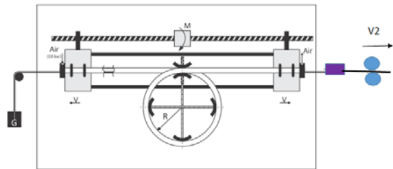
Fig. 5. An example of test stand to measurements sliding friction in medical devices catheter and guide
