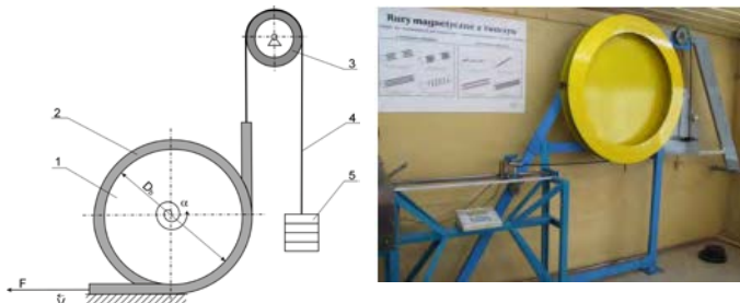
Fig. 3. The scheme and the laboratory test machine to measure coefficient of friction: 1 – measuring drum, 2 – duct, 3 – roller, 4 – fiber optic cable, 5 – load; D_b – diameter of the measure drum, \alpha – wrapping angle of pipe around the drum, V – speed of the cable movement
