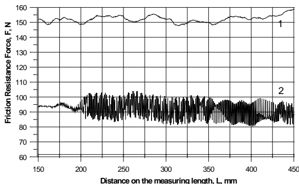
Fig. 4. The sample of diagram of the friction resistance force as the function of distance L ; 1-duct without slip layer on the inner surface, 2- duct with thin silicone slip layer on the inner surface. duct outside diameter 40 mm with triangular macro deviations, optotelecommunication cable (XOTKtd) outside layer made of PE-HD
