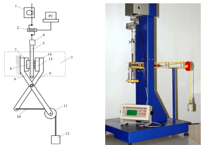
Fig. 2. The scheme and the laboratory test machine to measure coefficient of friction on specifically length with one-sided sliding
