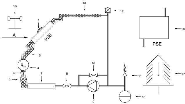
Fig. 2 Scheme of the measuring line.
