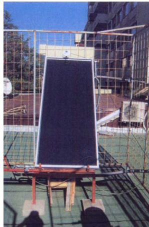
Fig. 3 Part of the measuring line for hydraulic and thermotechnical tests of solar thermal panel.
