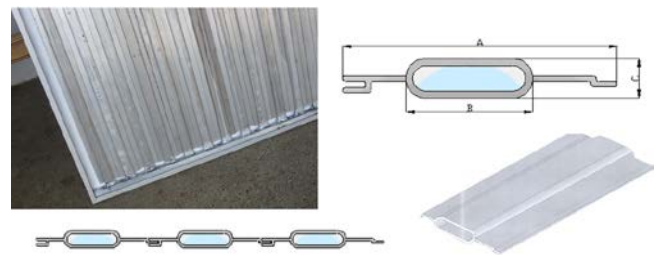
Fig. 1 Absorber surface of solar panel with a schematic connection of absorber lamellae (cross-section).
