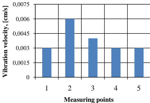
Figure 5. Graphic presentation of the vibration velocities at the five specific measuring points
