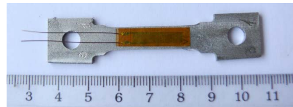
Fig. 4. SLM tensile test specimen with strain gauge.
