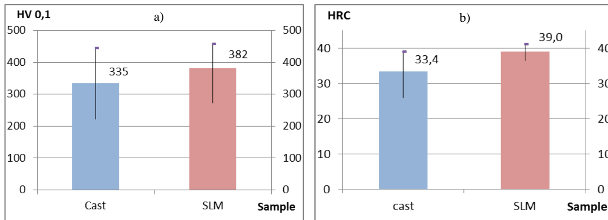
Fig. 7. Vickers hardness: a) and Rockwell hardness; b) of samples produced by casting and SLM.
