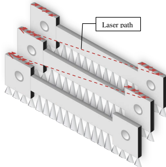
Fig. 2. Scheme of tensile test specimens' production by SLM
