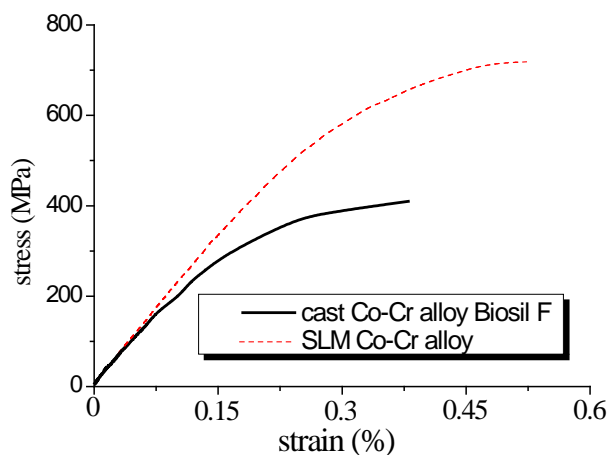
Fig. 8. Typical stress – strain curves for both specimen groups.
