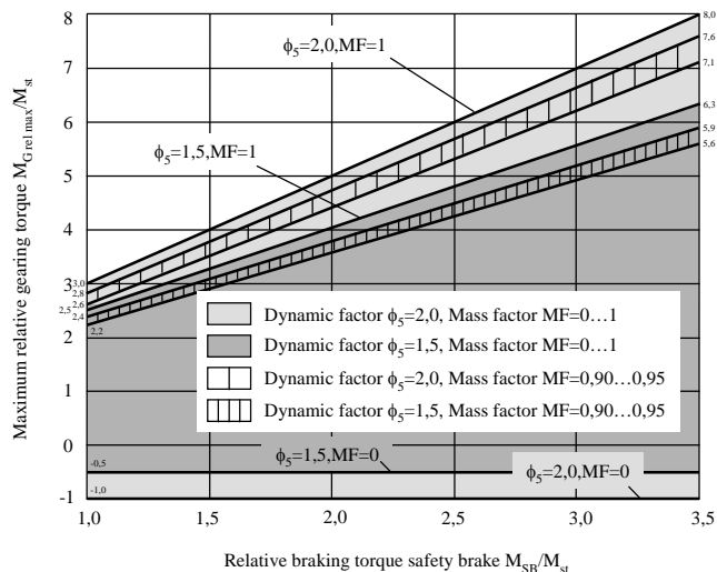
Fig. 5 Maximum relative gearing torque
