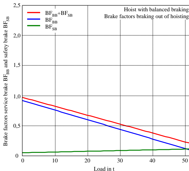
Fig. 7 Braking factors for braking out of hoisting
